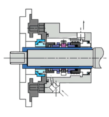
Double Pusher Seal (DROTT)
