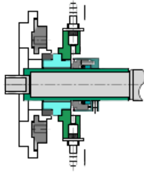
Single Pusher Seal (RA)
